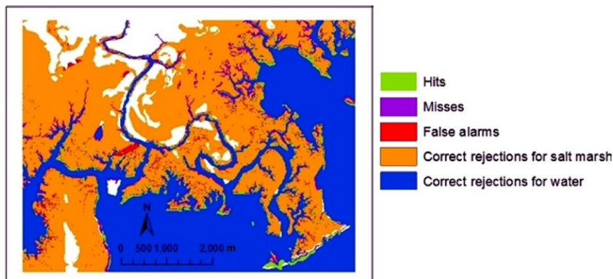
FIGURE 3 Agreement and disagreement of our 2007 simulations compared to the national wetland inventory (NWI) data of 2007 in reference to 1988 NWI data
