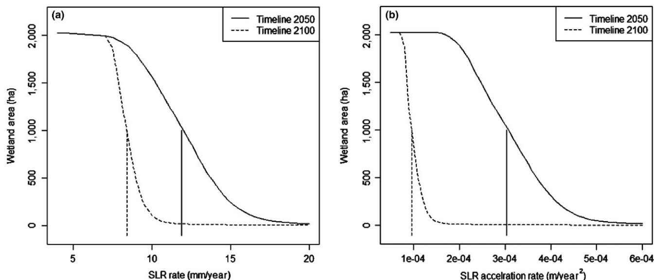
FIGURE 4 Coastal wetland area for 2050 and 2100 at different sea-level rise (SLR) rates (a) and different SLR acceleration rates (b). The vertical lines showed the thresholds of SLR rate and SLR acceleration rate for 2050 and 2100, respectively
