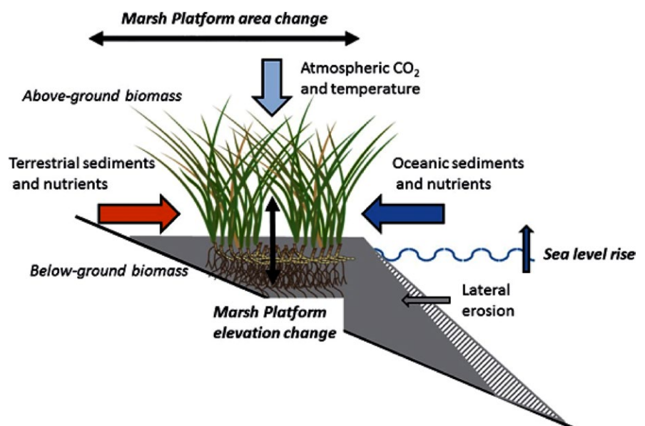
FIGURE 1 Conceptual model indicating model elements simulated that affect marsh platform elevation and area in response to sea-level rise (SLR) and climate change drivers. Sustainable marsh platforms require plant biomass and sediment deposited from water column to maintain a positive increase in elevation that meets or exceeds the rates of SLR
