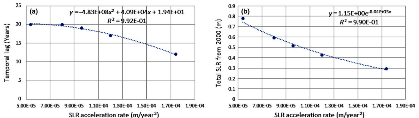
FIGURE 6 (a) The temporal lag before the total area of coastal wetlands starts to decrease substantially after the threshold of SLR rate is exceeded versus acceleration rate of sea-level rise (SLR). (b) The total SLR sustained since 2000 that coastal wetlands can take before the total area of coastal wetland starts to decrease substantially versus acceleration rate of SLR. (Note: intermediate-low scenario has acceleration rate of 5.42 \times 10^{-5} m/year 2 , and intermediate-high emission scenario has acceleration rate of 1.74 \times 10^{-4} m/year 2 )
