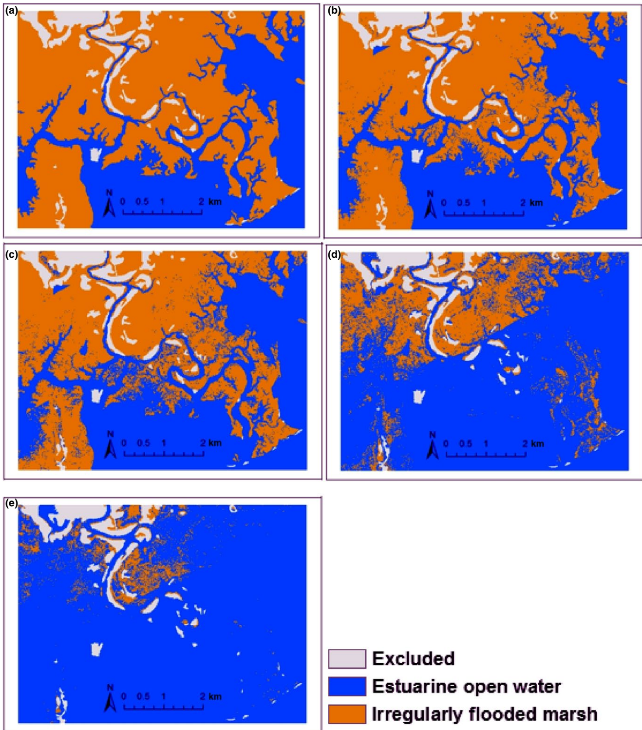
FIGURE 5 Wetland distribution in (a) 1988, (b) 2100 under the sea-level rise (SLR) rate of 4 mm/year (current), (c) 2100 under the SLR rate of 7.5 mm/year (~ 1 mm/year lower than the threshold of SLR rate), (d) 2100 under the SLR rate of 8.5 mm/year (~ the threshold of SLR rate), and (e) 2100 under the SLR rate of 9.5 mm/year (~1 mm/year above the threshold of SLR rate)
